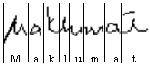
Figure 1: Recognizing "Maklumat"
