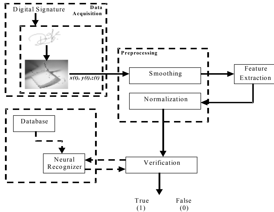
Figure 7 : System Architecture
